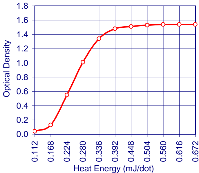
Dynamic Sensitivity
