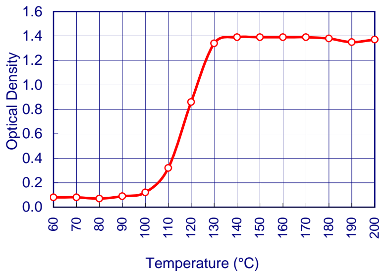
Static Sensitivity
