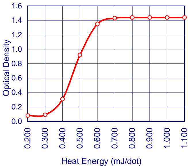
Dynamic Sensitivity
